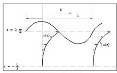
Figure B-6-2. Variation of particle velocity with depth (open 1986) Coastal Engineer Manual (CEM)
