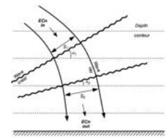
Fig. 4.11 Schematic diagram of depth-based wave refraction. Wave rays are shown perpendicular to the wave crests, which indicates the direction of wave propagation. See text for further explanation.
