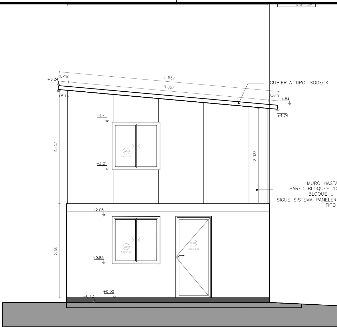
FACHADA PRINCIPAL ESCALA_1/50
