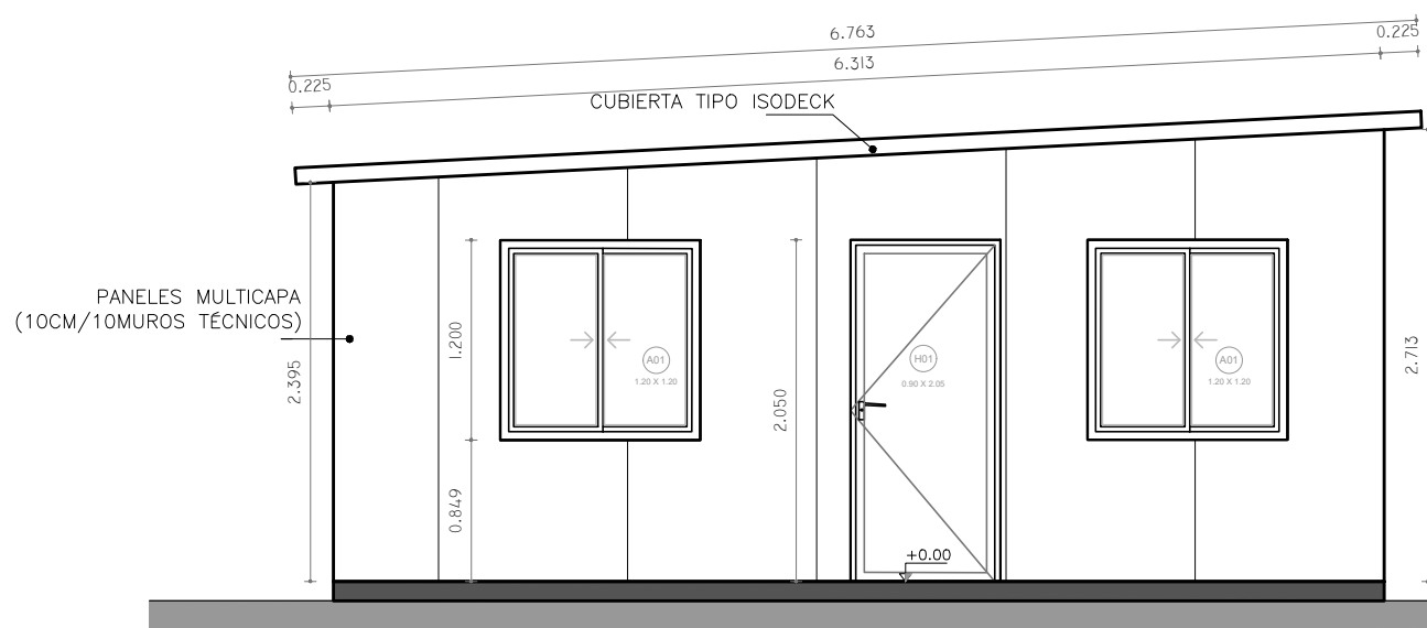
FACHADA PRINCIPAL ESCALA_1/50
